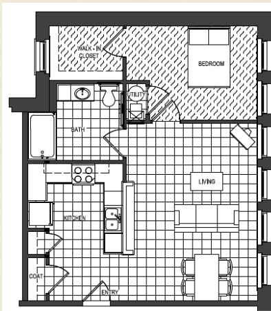
TYPE C ONE BEDROOM 648 SQ. FT.
